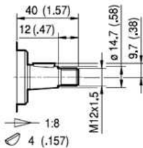
TO Coppia Max Max Torque 145 Nm
